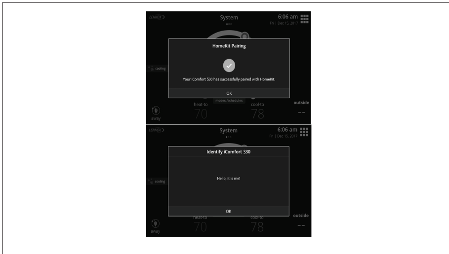
Figure 29. Pairing Successful
