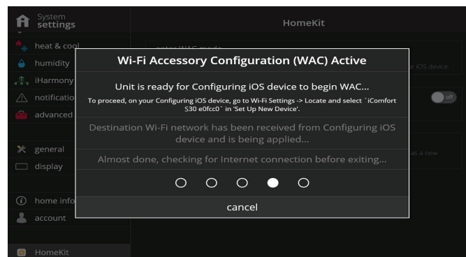
Figure 24. Wi-Fi Configuration
