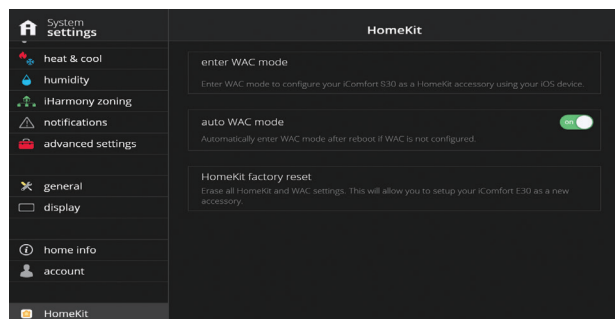
Figure 22. HomeKit Menu
