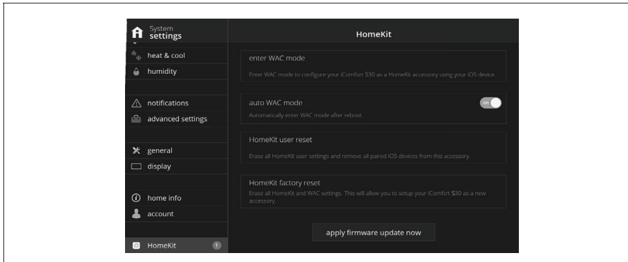
Figure 30. HomeKit Menu
