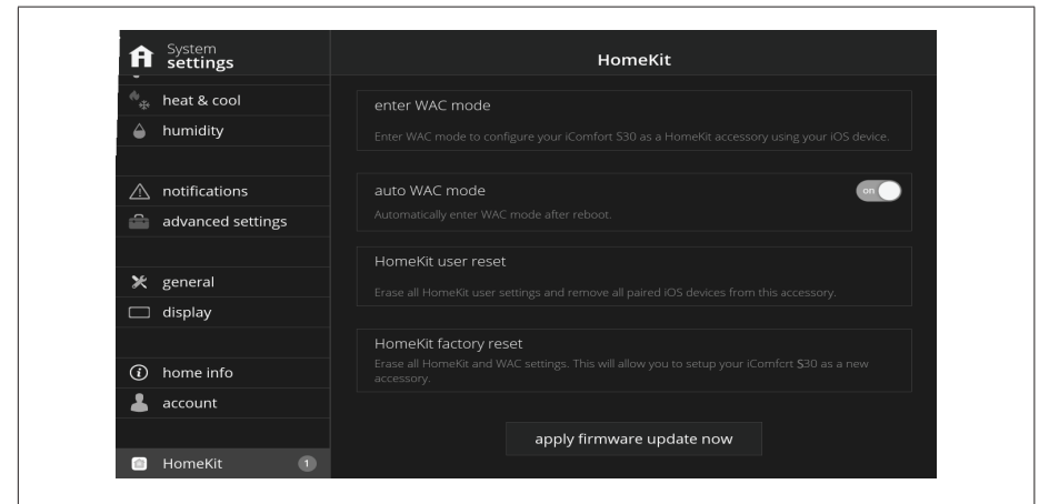
Figure 33. HomeKit Notification
