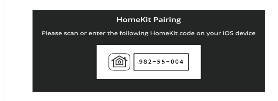
Figure 28. Pairing Code
